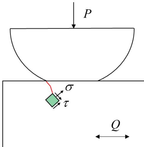
Fig. 7. Sketch of the stress evaluation ahead of the crack tip.
