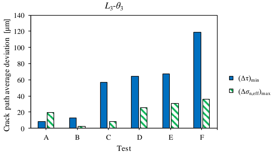
Fig. 11. Average deviation of the selected crack direction criteria at the end of L_3-\theta_3 segment.
