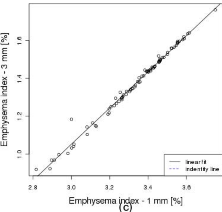
Standardized dataset
