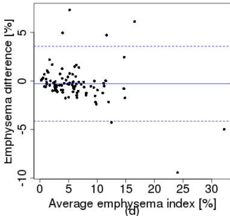
Bland-Altman plot
