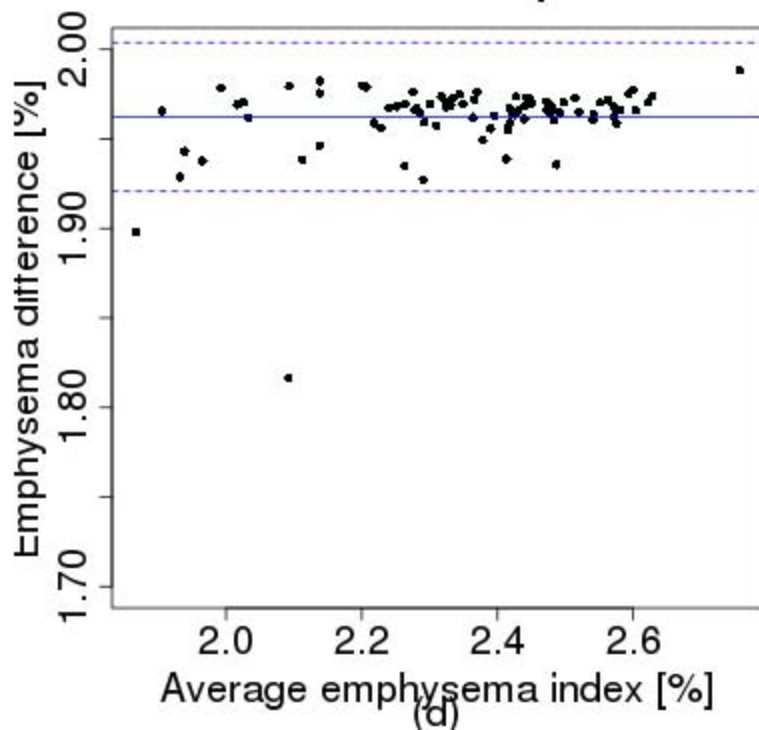
Bland-Altman plot
