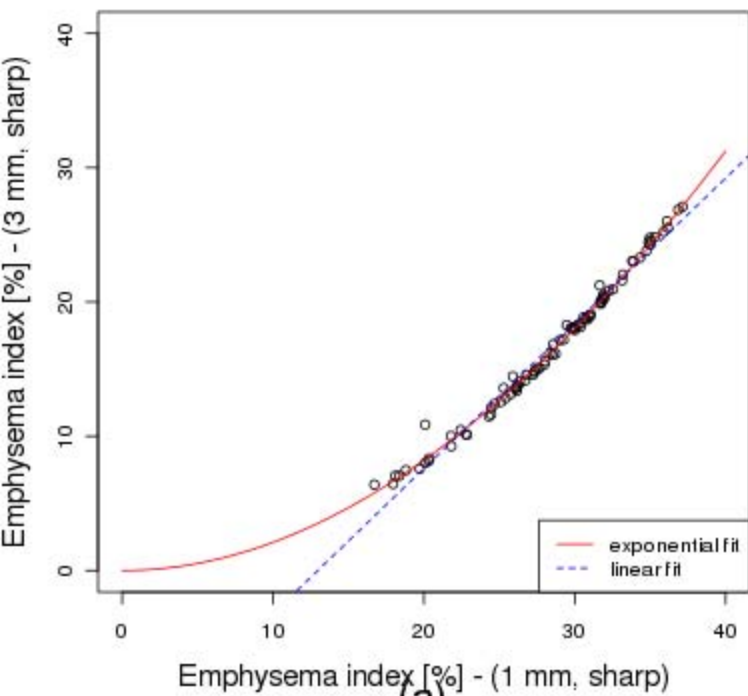
Standardized dataset
