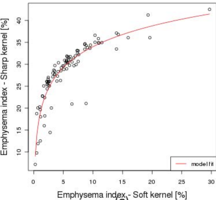
Standardized dataset
