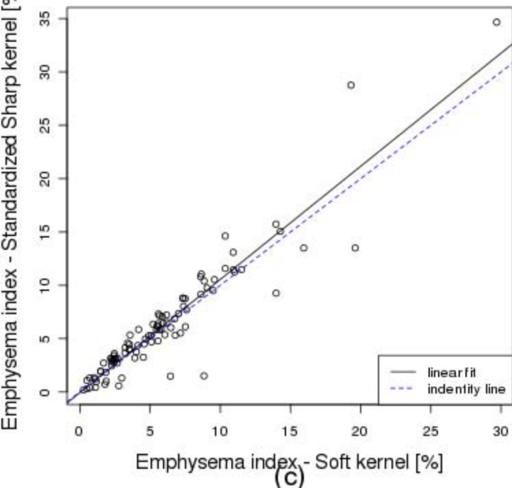
Standardized dataset
