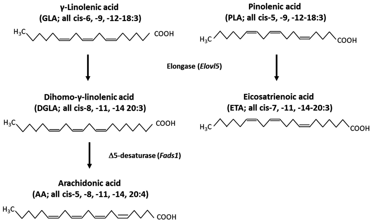
Figure 1. The pathway of metabolic conversion of gamma-linolenic acid and the likely pathway of conversion of pinolenic acid to longer-chain polyunsaturated fatty acids. Genes encoding the various enzymes are shown in brackets.
