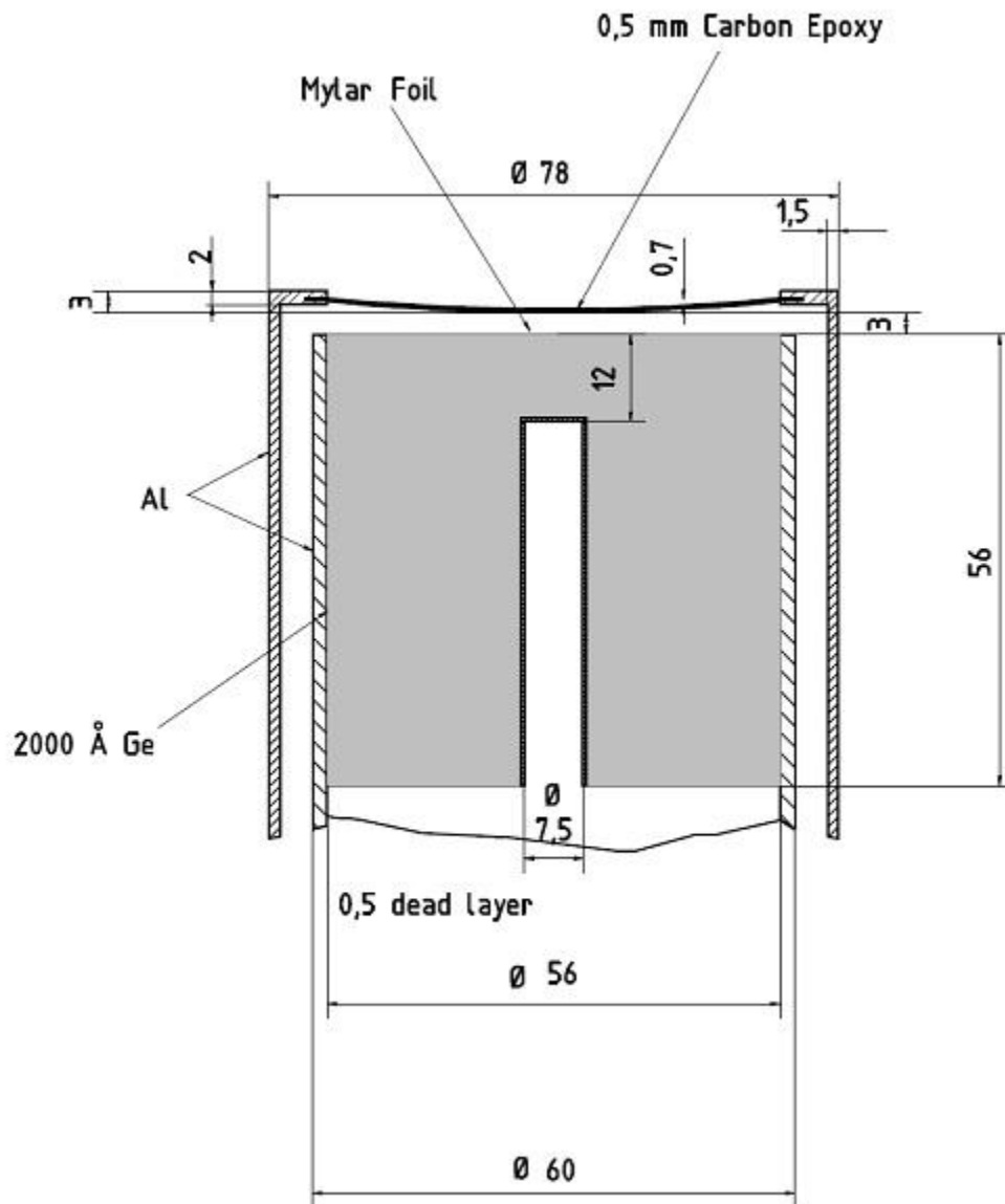
Fig. 1. Cross-section of the detector with the dimensions and materials provided by the manufacturers.
