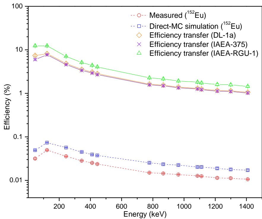
Fig. 2. Measured and computed (MCNPX) photo-peak efficiency. The dotted lines correspond to the experimental efficiency for the reference source and the calculated efficiency by direct MC simulation using the nominal parameters of the detector. The solid lines represent the efficiency after application the efficiency transfer.
